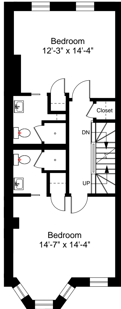
Second Floor Plan Ceiling Height = 9'-0"
