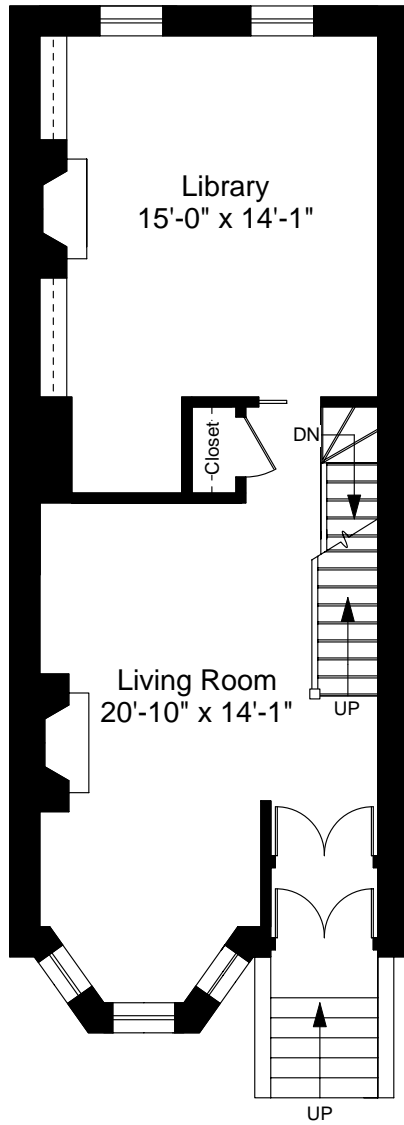
First Floor Plan Ceiling Height = 10'-0"
