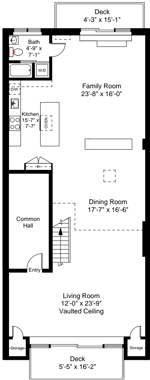
First Floor Plan Ceiling Height = 9'-9"
