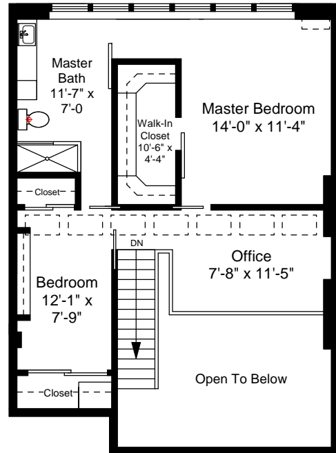
Second Floor Plan Ceiling Height = 8'-0"
