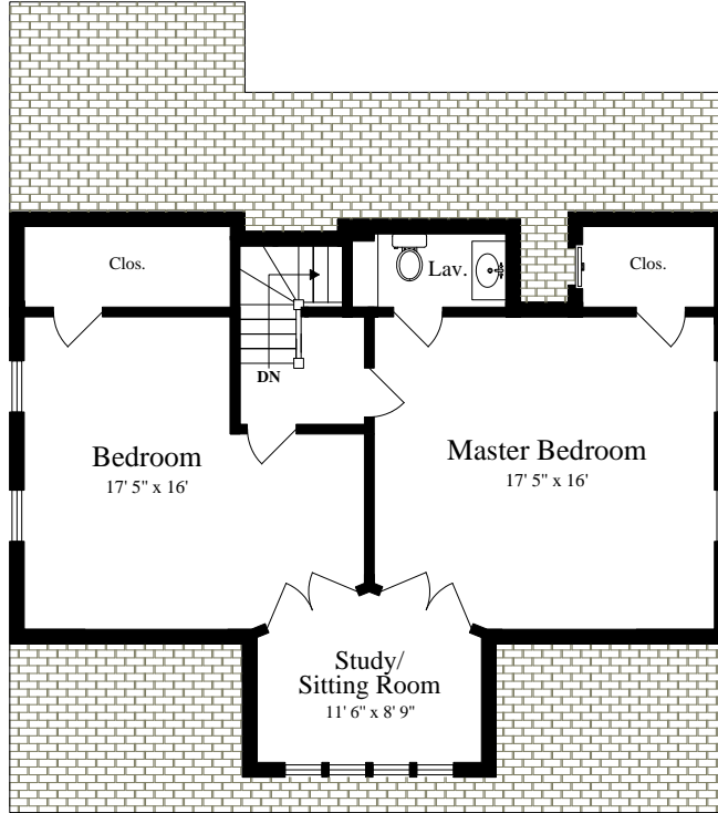
SECOND FLOOR (ceiling = 7' 5")
