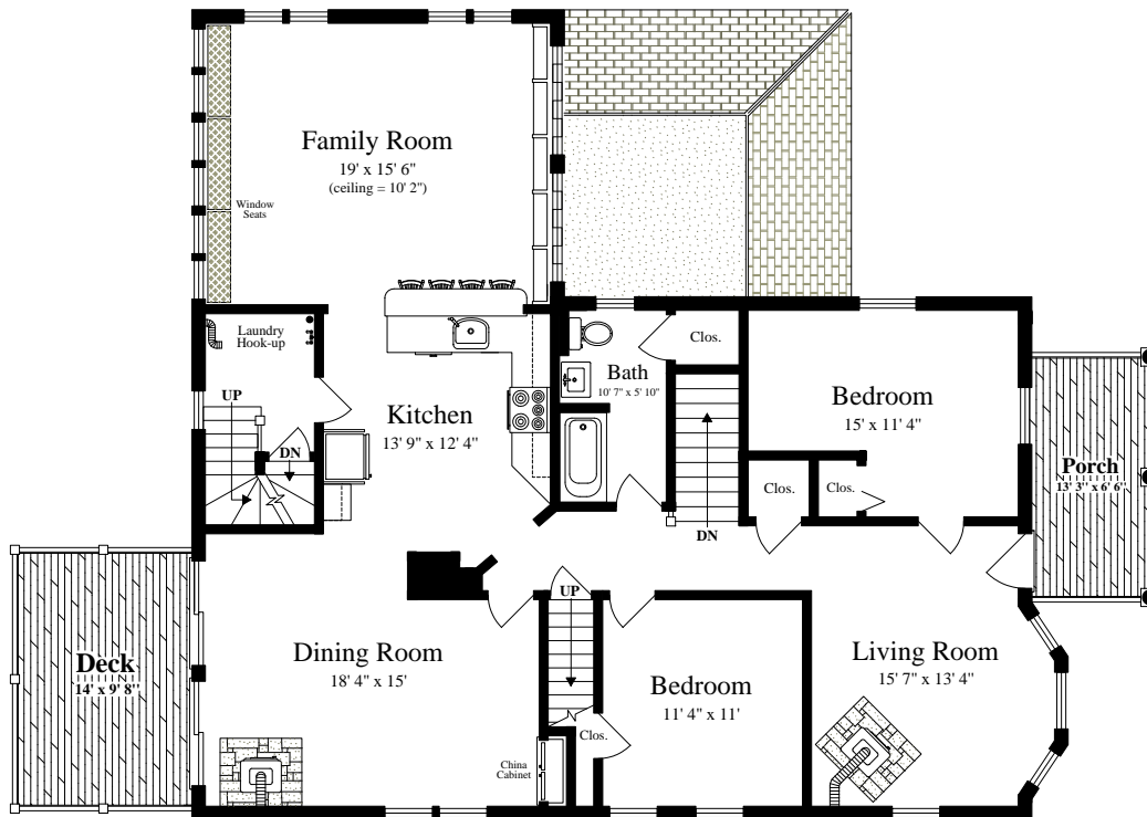
SECOND FLOOR (ceiling = 8' 3")
