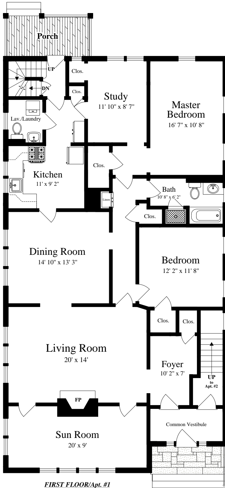
FIRST FLOOR/Apt. #1 (ceiling = 8')
