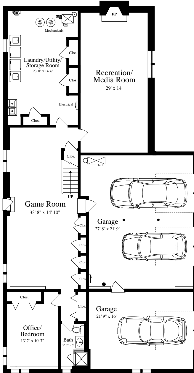
LOWER LEVEL (ceiling = 6' 9")
