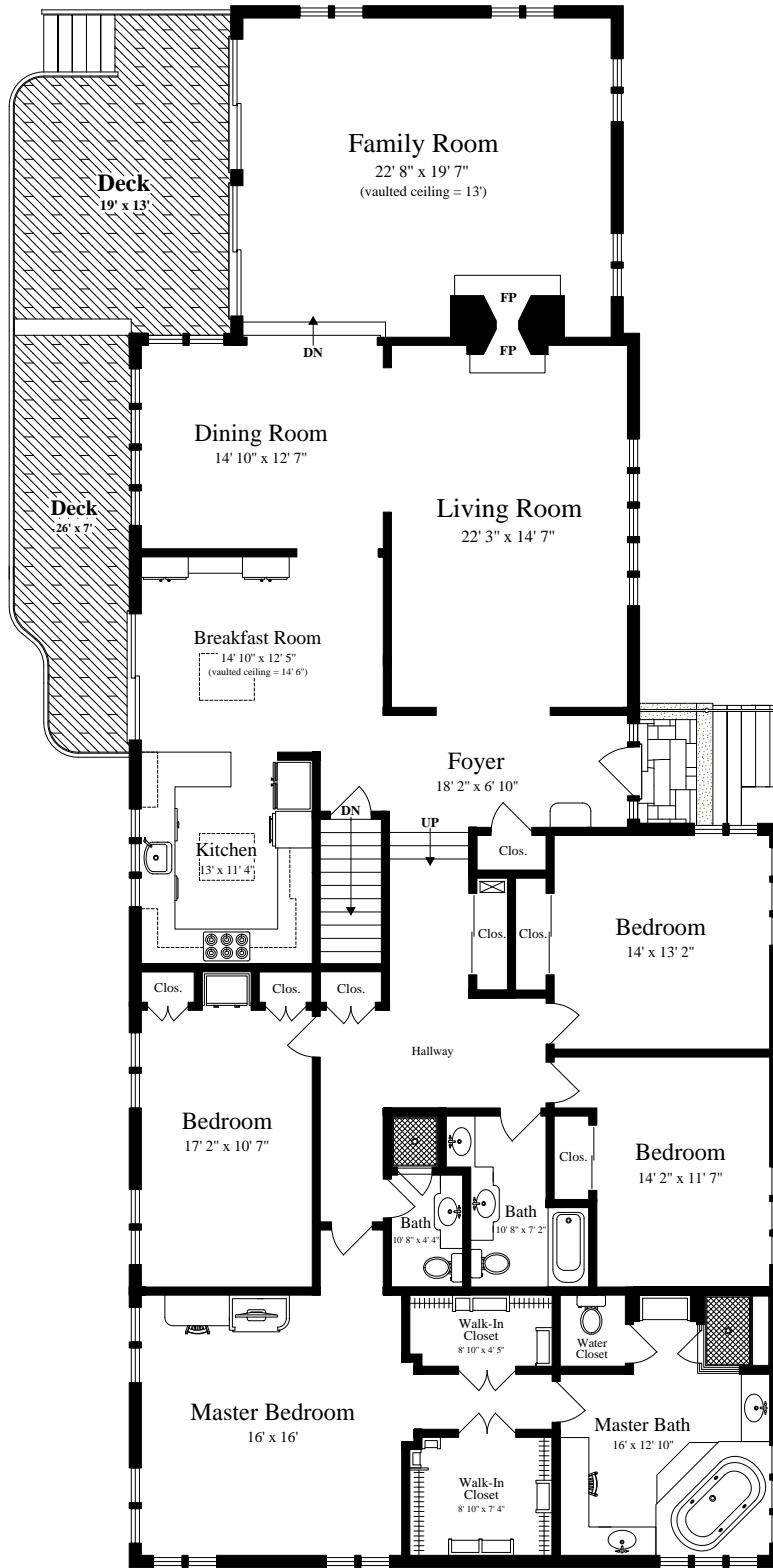
FIRST FLOOR (ceiling = 8')
