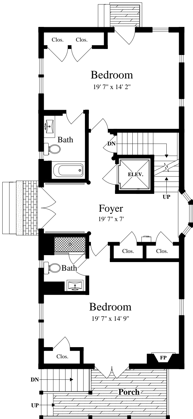
FIRST FLOOR (ceiling = 8' 9")
