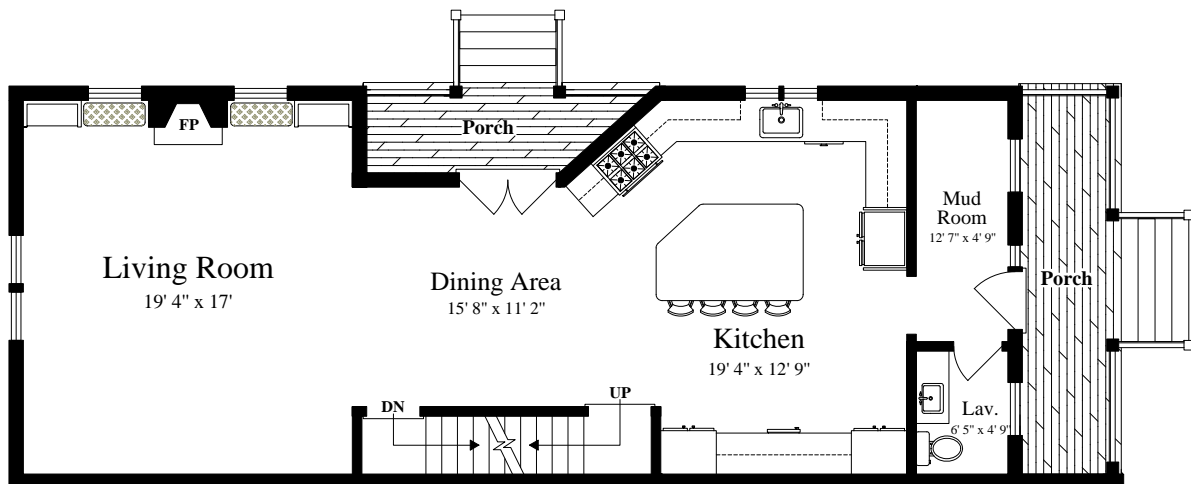
FIRST FLOOR (ceiling = 9')
