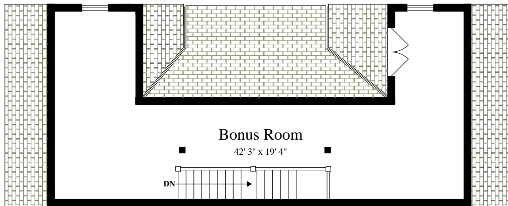
THIRD FLOOR (ceiling = 7' 2")
