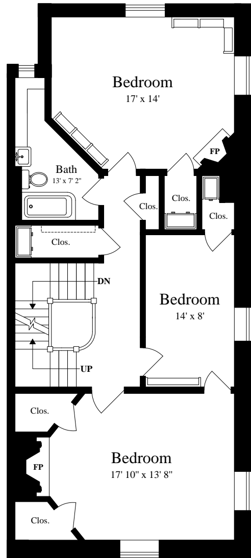
SECOND FLOOR (ceiling = 9' 6")
