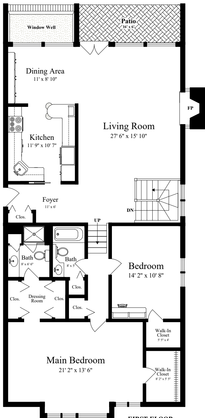
FIRST FLOOR (ceiling = 8')
