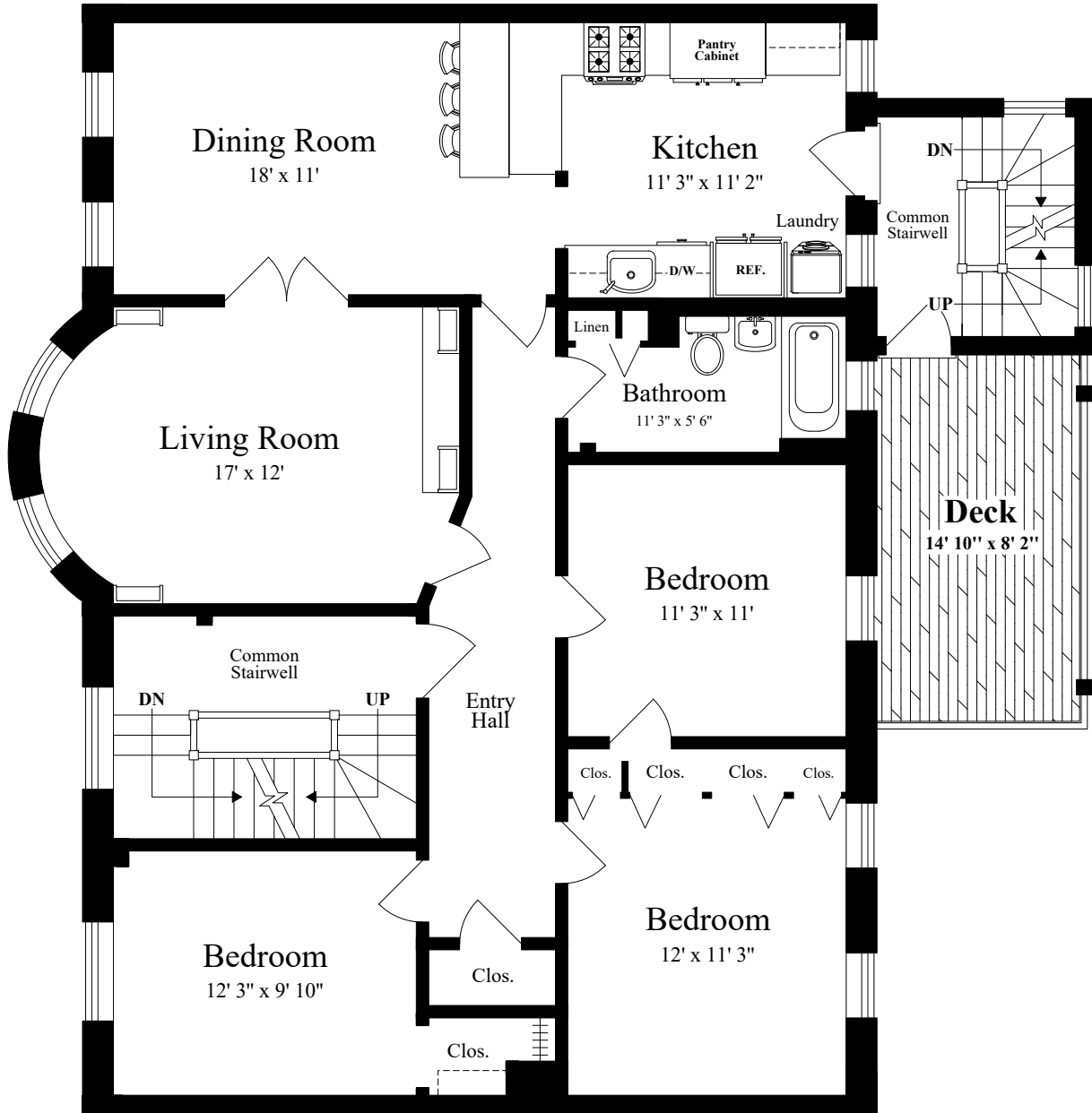
SECOND FLOOR (ceiling = 8' 10")
