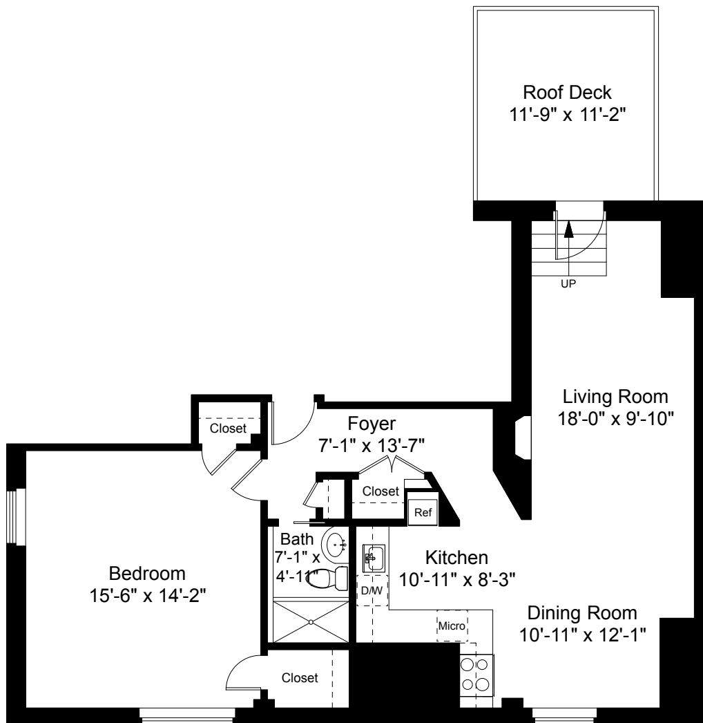
Unit 91 Floor Plan Ceiling Height = 8'-4"
