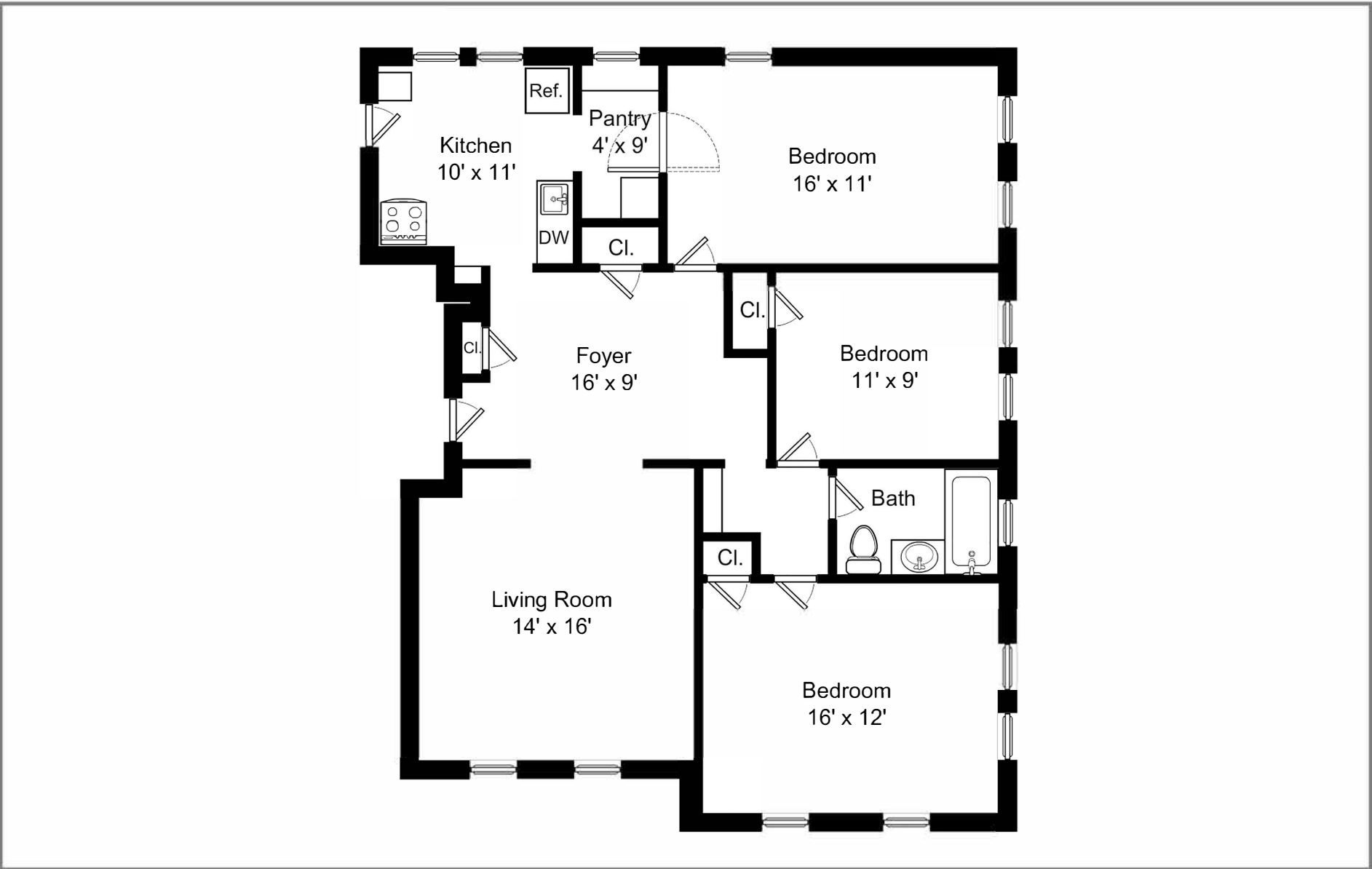
3 Greenway Court, Unit 1 Floor Plan
