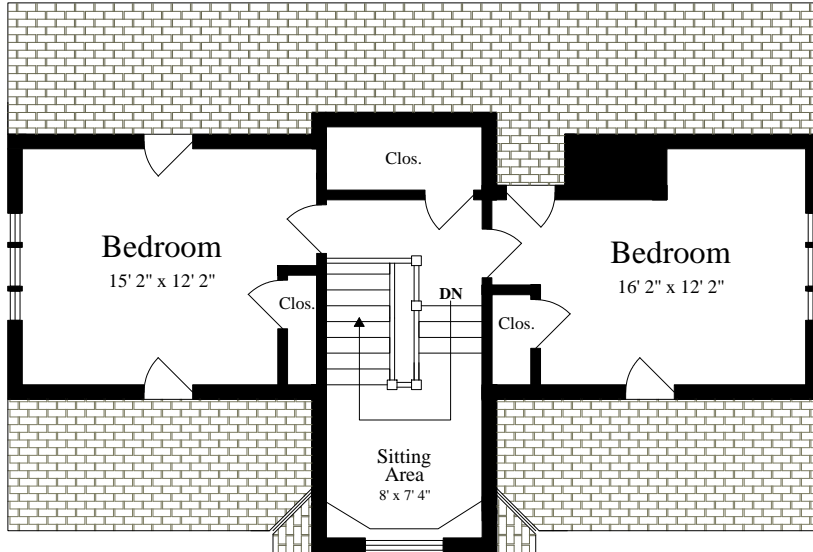
THIRD FLOOR (ceiling = 7' 5")
