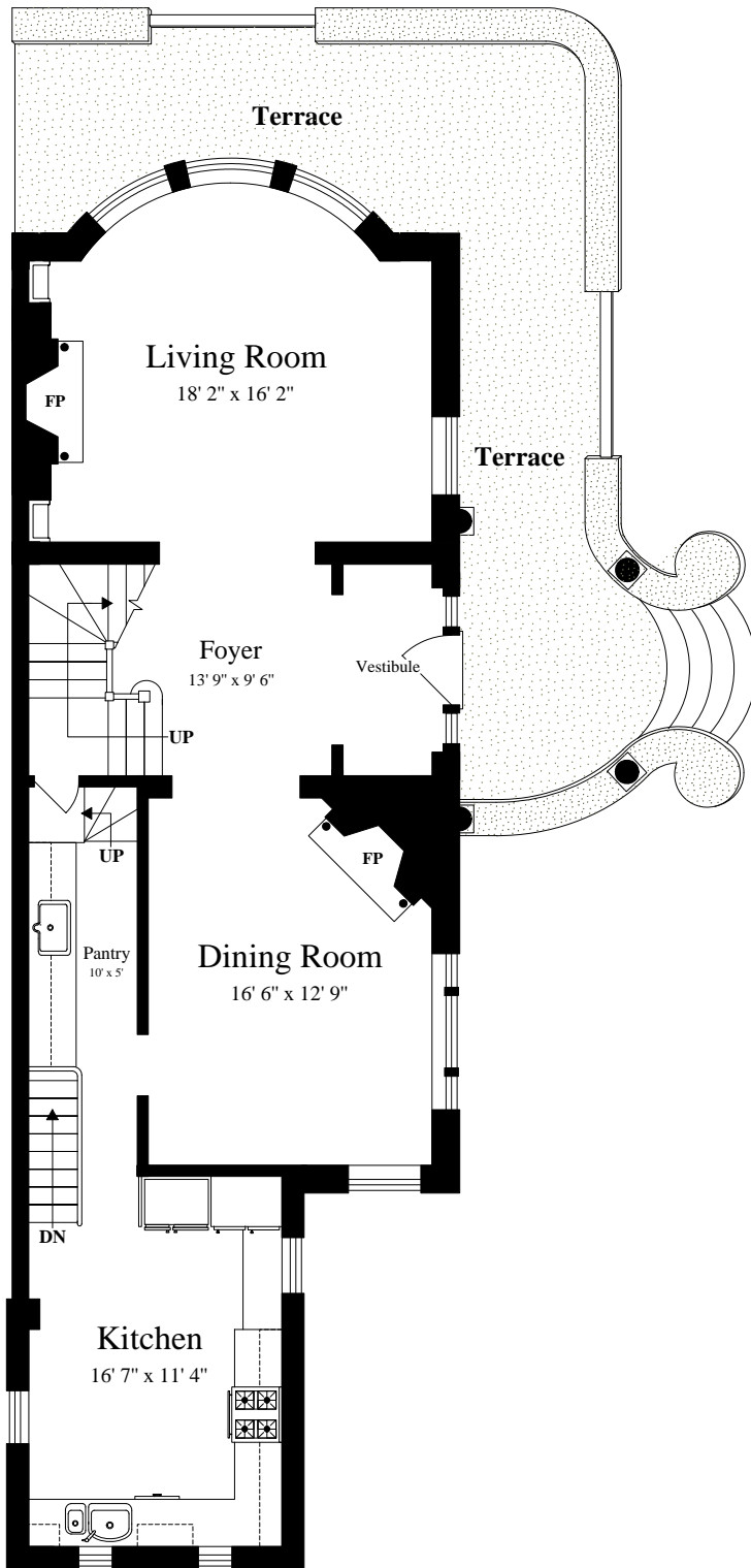
FIRST FLOOR (ceiling = 9')
