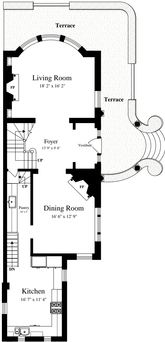
FIRST FLOOR (ceiling = 9')
