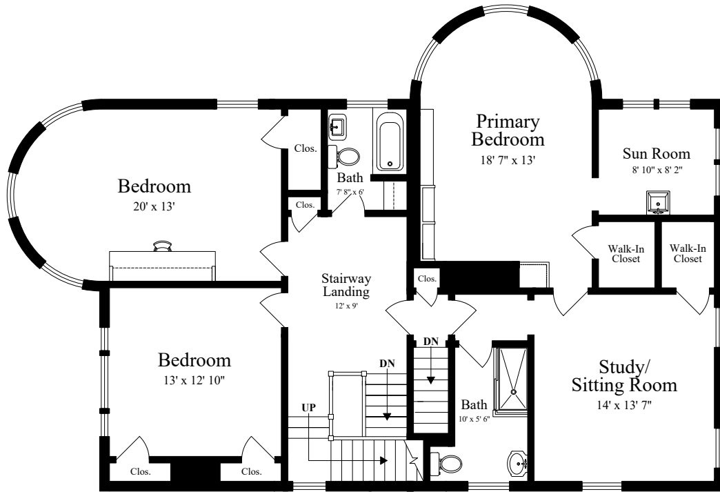
SECOND FLOOR (ceiling = 8' 6")
