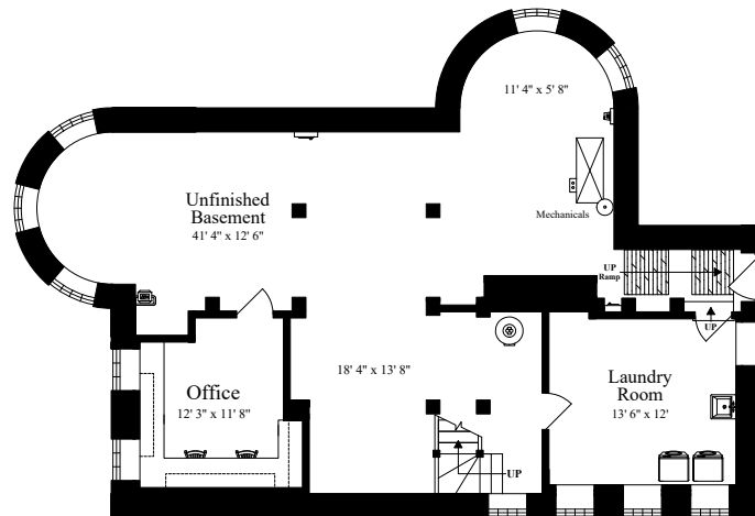
LOWER LEVEL (ceiling = 8')
