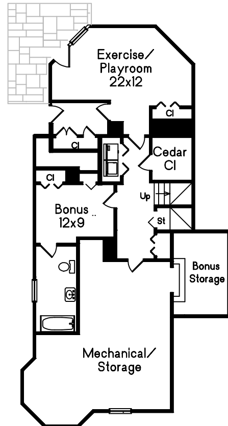
Lower Level
