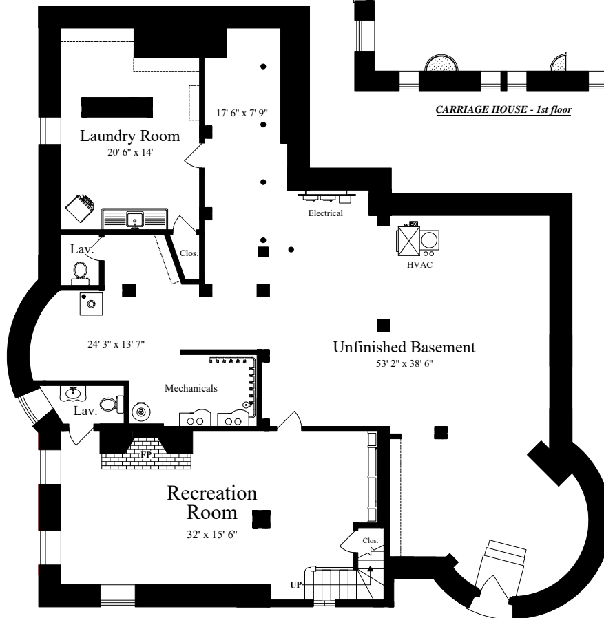
LOWER LEVEL (ceiling = 8' 6")
